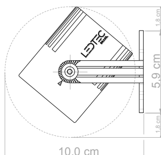
VISTA FRONTAL
